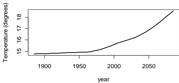
Figure 3. Global annual mean surface temperature (°C) for the CSIRO Mark 2 GCM.
